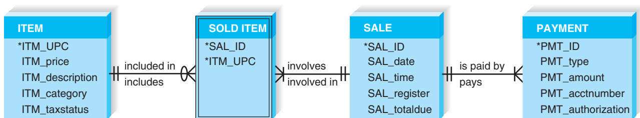
FIGURE 6-1 Supermarket ERD
