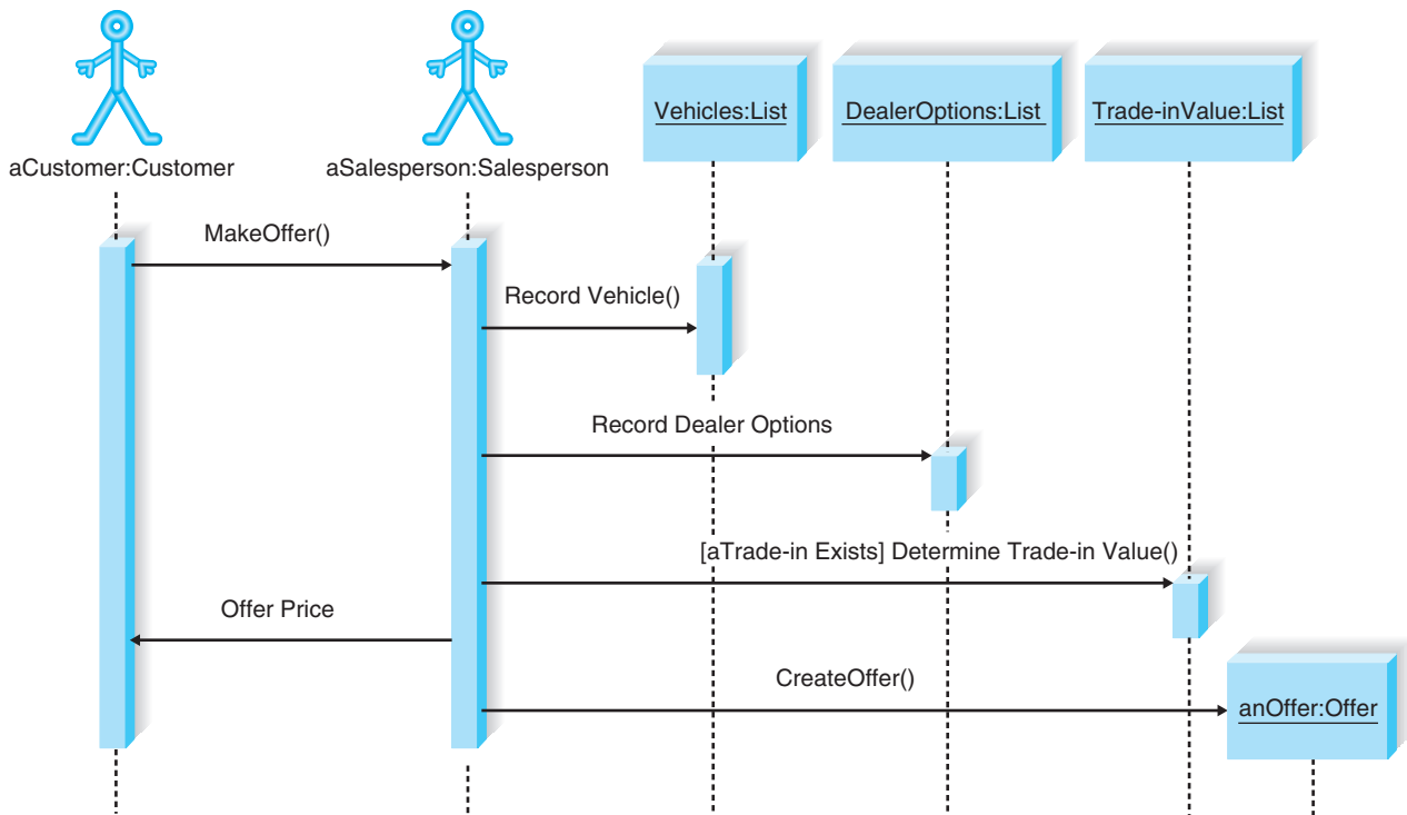
FIGURE 14-22 Sequence Diagram
