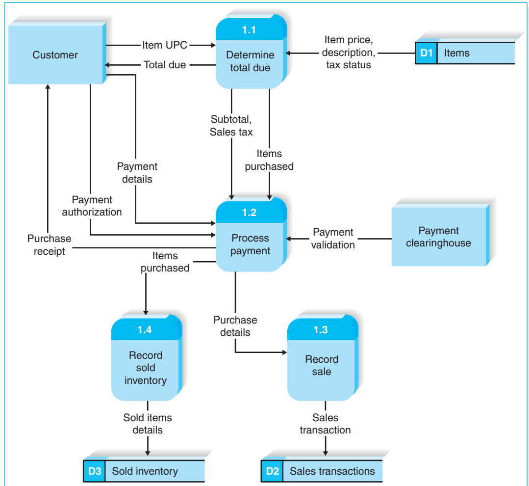
FIGURE 5-1 Supermarket Checkout DFD
