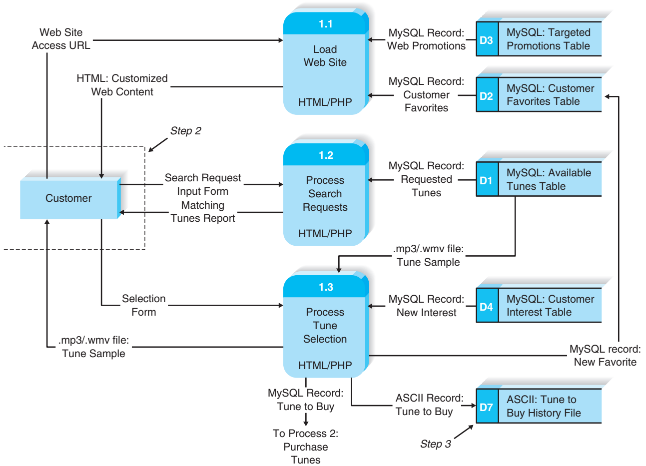
FIGURE 10-2 Physical DFD for Tune Source Process 1: Search and Browse Tunes (the How)
