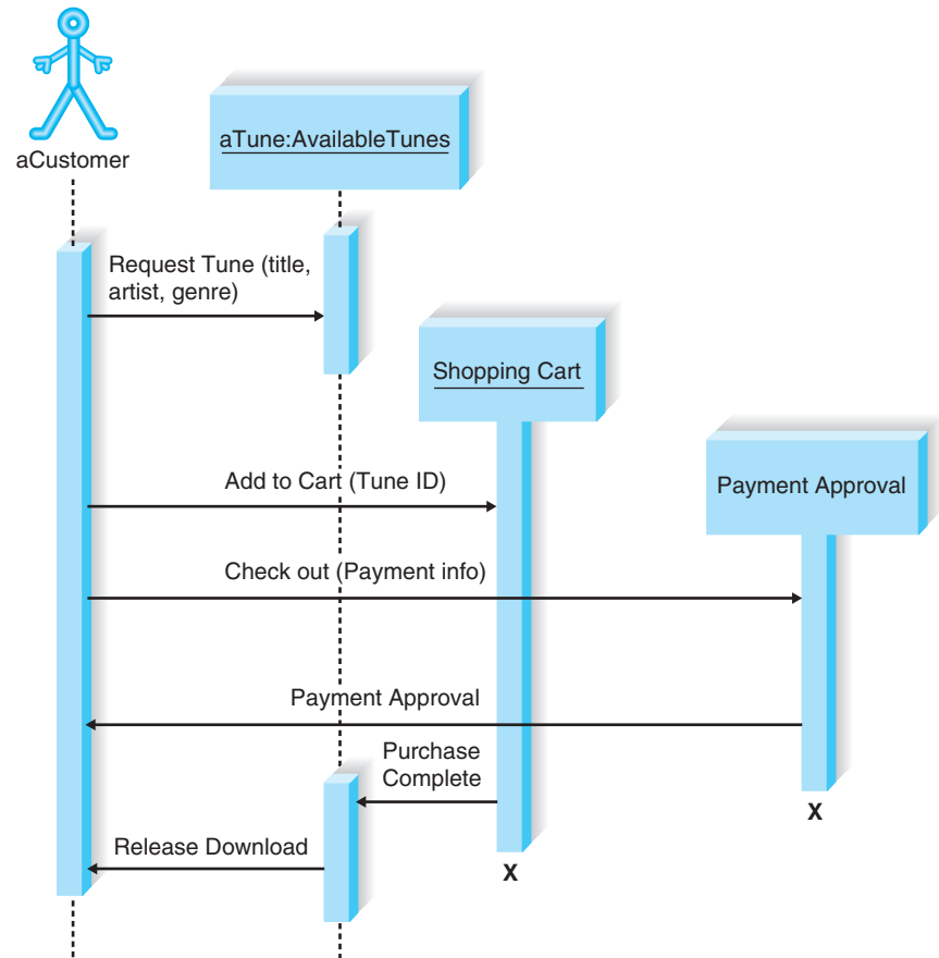
FIGURE 14-25 Sequence Diagram for Purchase Tunes Scenario
