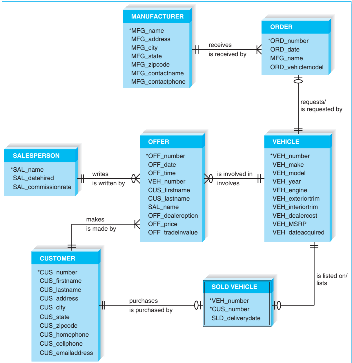
FIGURE 6-11 Holiday Travel Vehicles ERD
