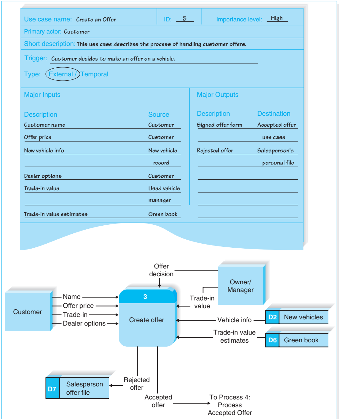
FIGURE 5-6 Holiday Travel Vehicles Process 3 DFD Fragment
