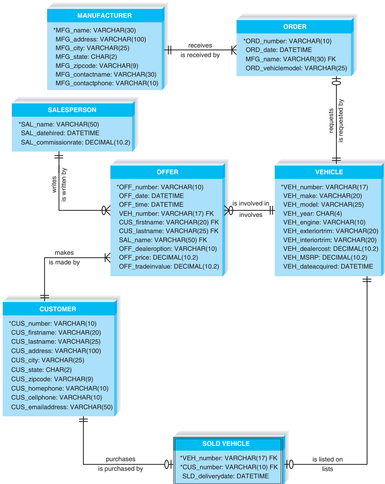
FIGURE 11-11 Holiday Travel Vehicle Physical ERD
