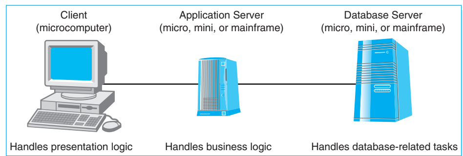
FIGURE 8-4 Three-Tiered Client-Server Architecture
