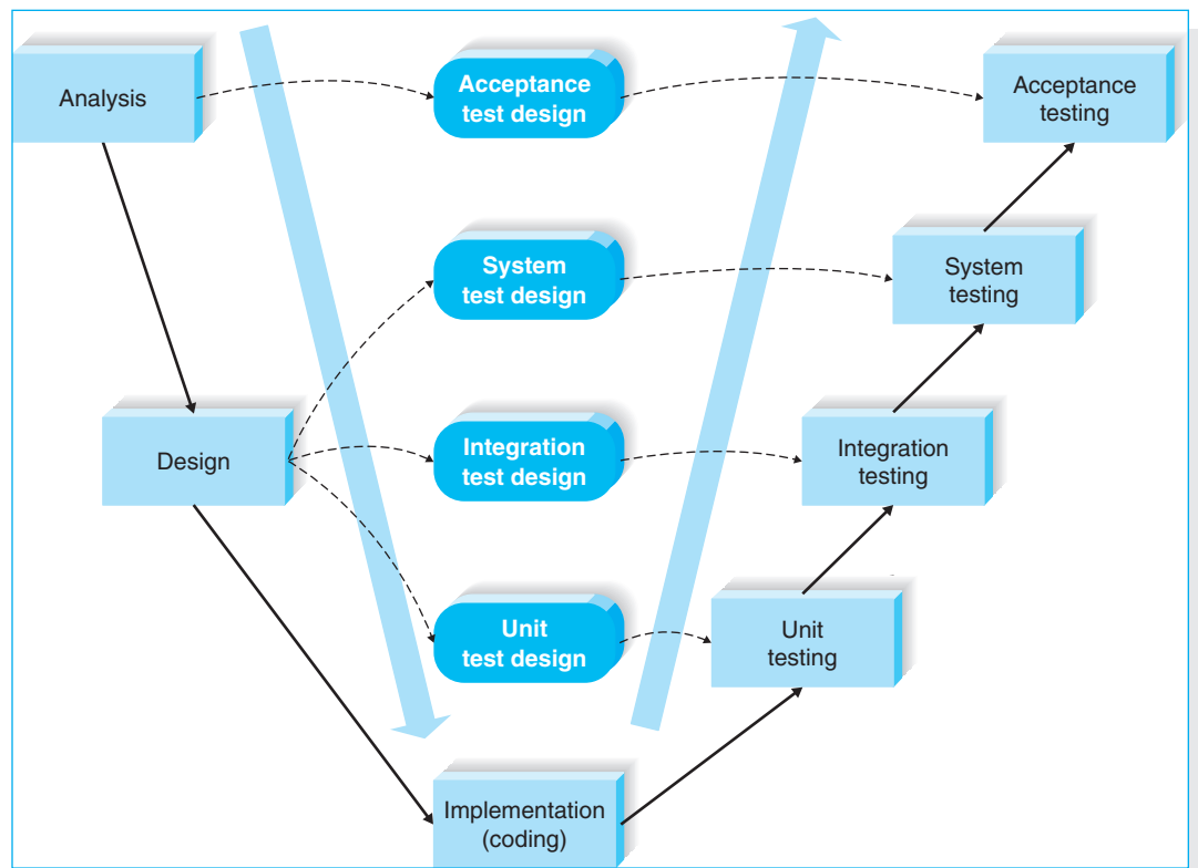
FIGURE 2-4 V-Model
