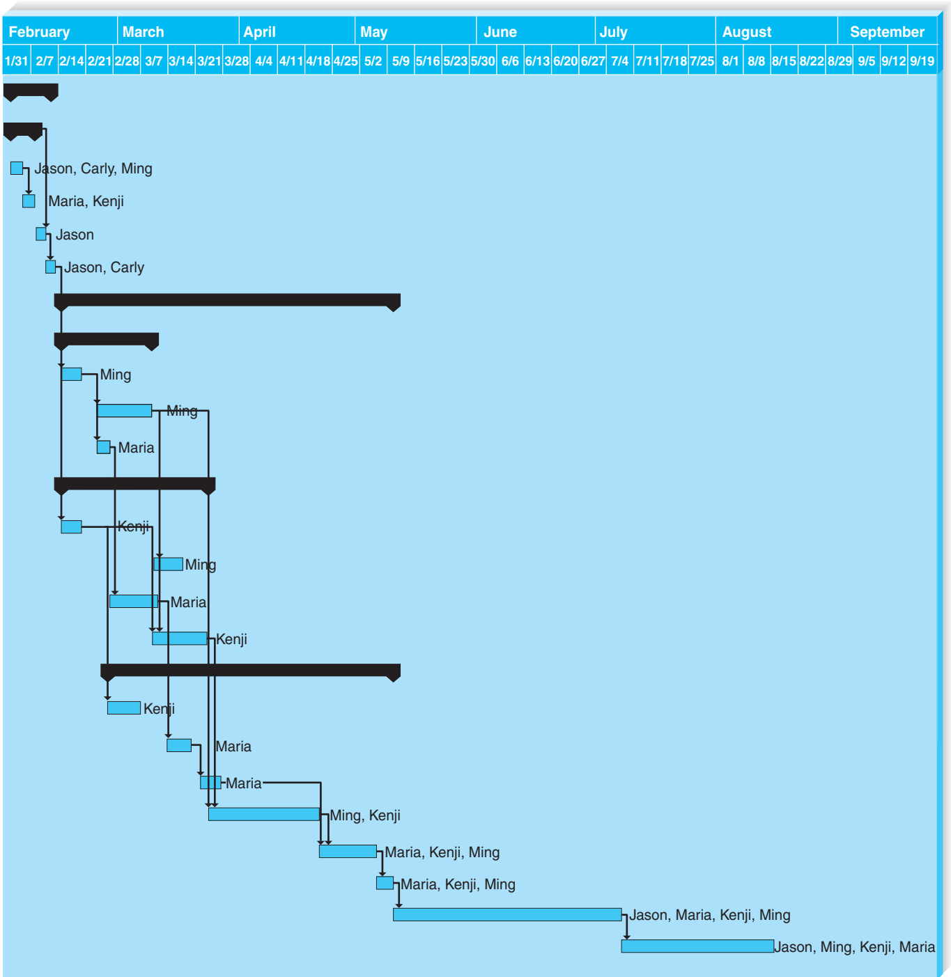
FIGURE 2-23 Gantt Chart
