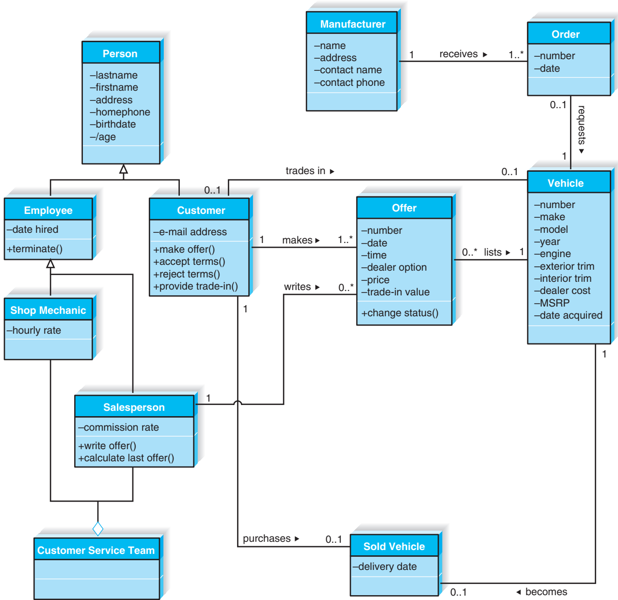
FIGURE 14-16 Class Diagram for Holiday Travel Vehicles
