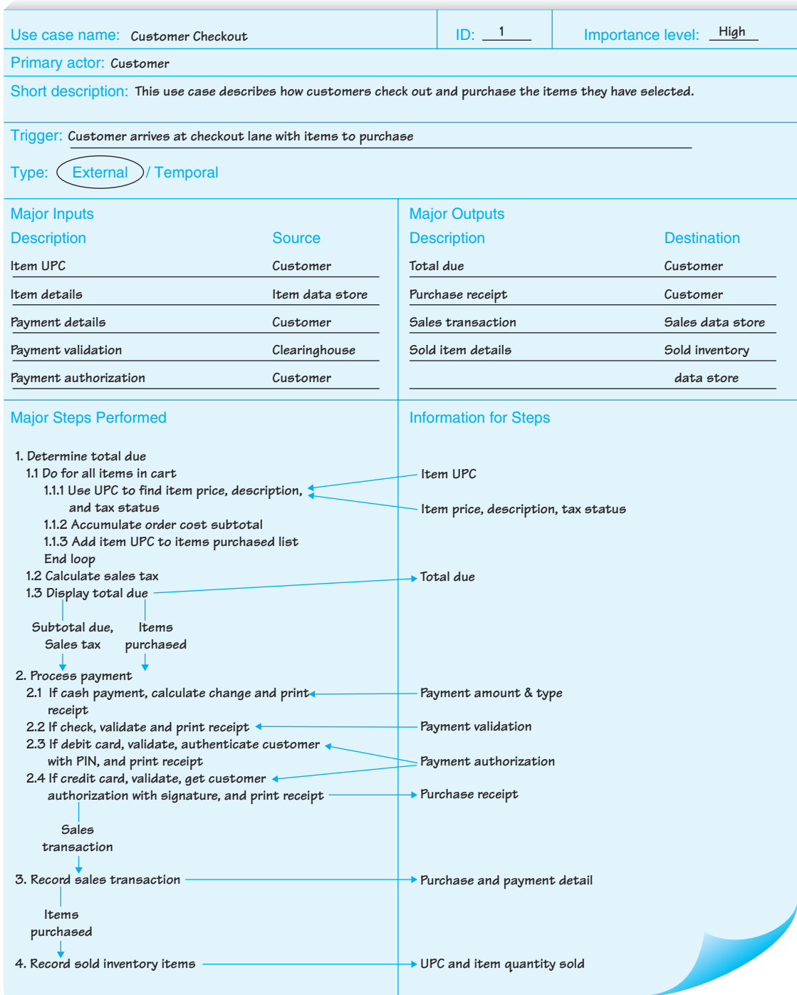
FIGURE 4-1 Supermarket Checkout Use Case
