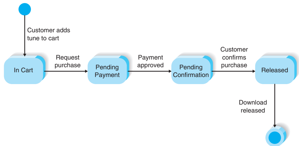
FIGURE 14-29 Behavioral State Machine Diagram for a Customer Purchase
