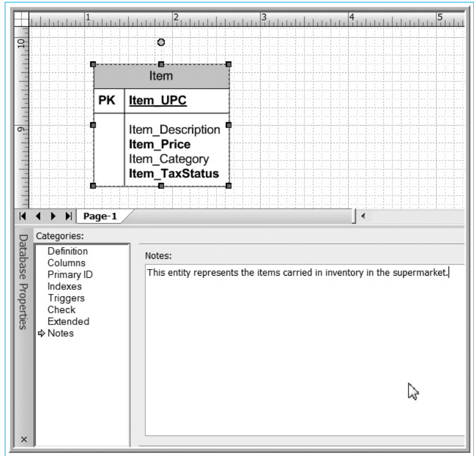
FIGURE 6-6 Data Dictionary Description for Item Entity (in Visio 2007)
