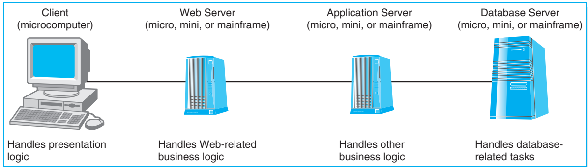
FIGURE 8-5 n-Tiered Client-Server Architecture
