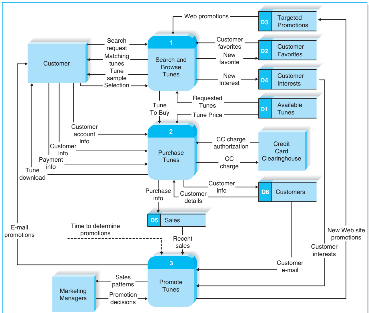
FIGURE 5-15 Tune Source Level 0 DFD
