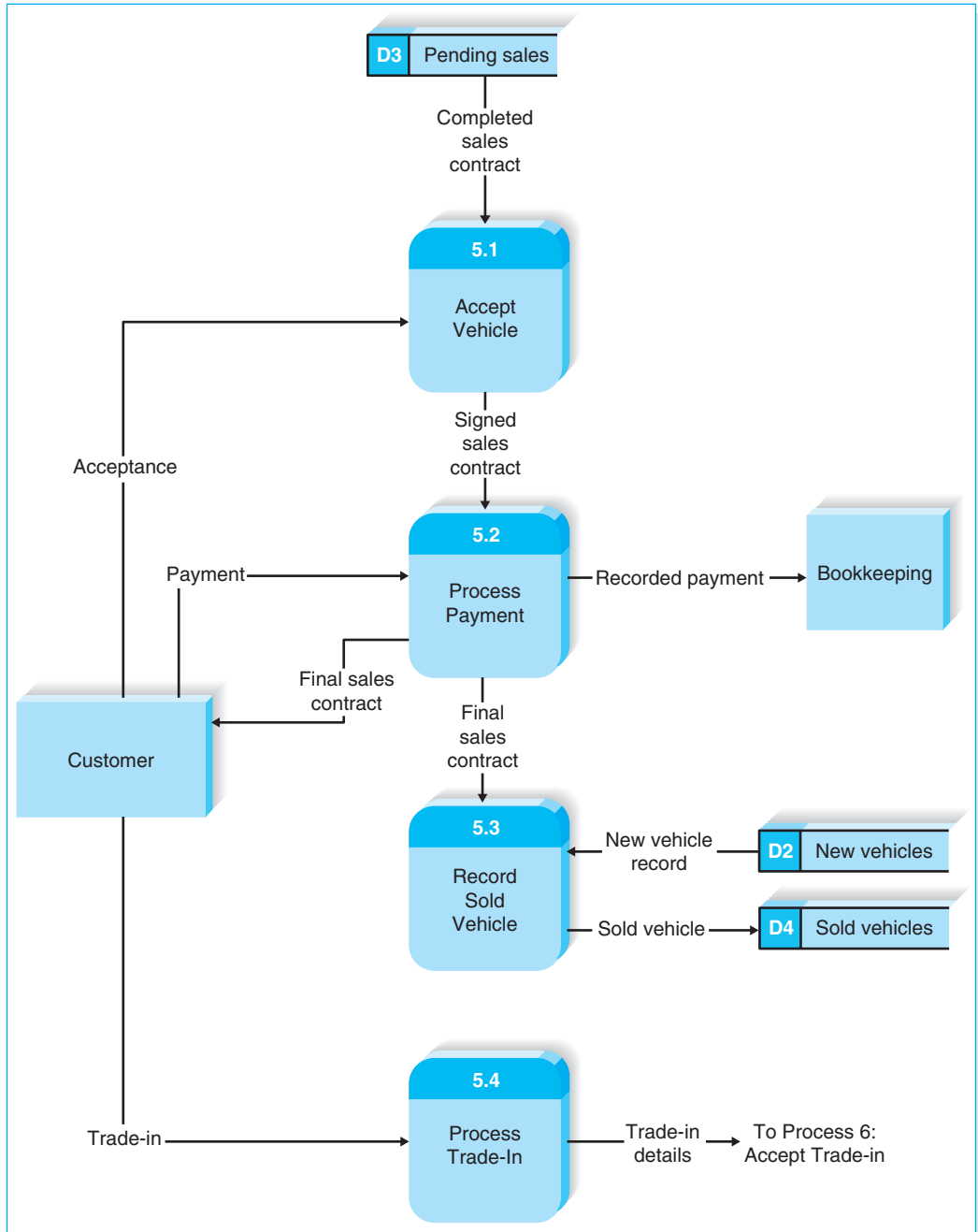
FIGURE 5-10 Level 1 DFD for Take Delivery of Vehicle
