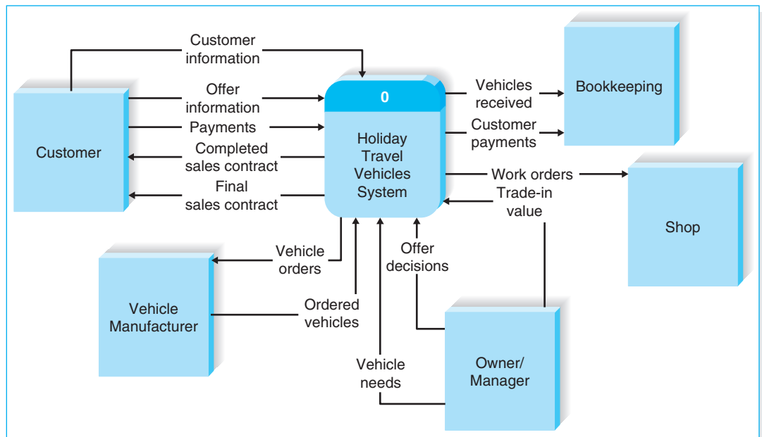
FIGURE 5-5 Holiday Travel Vehicles Context Diagram
