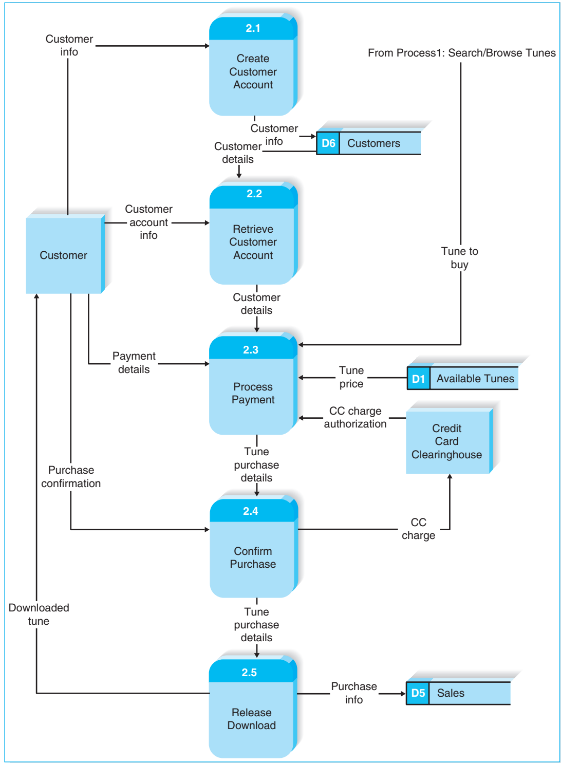
FIGURE 5-17 Level 1 DFD for Tune Source Process 2: Purchase Tunes
