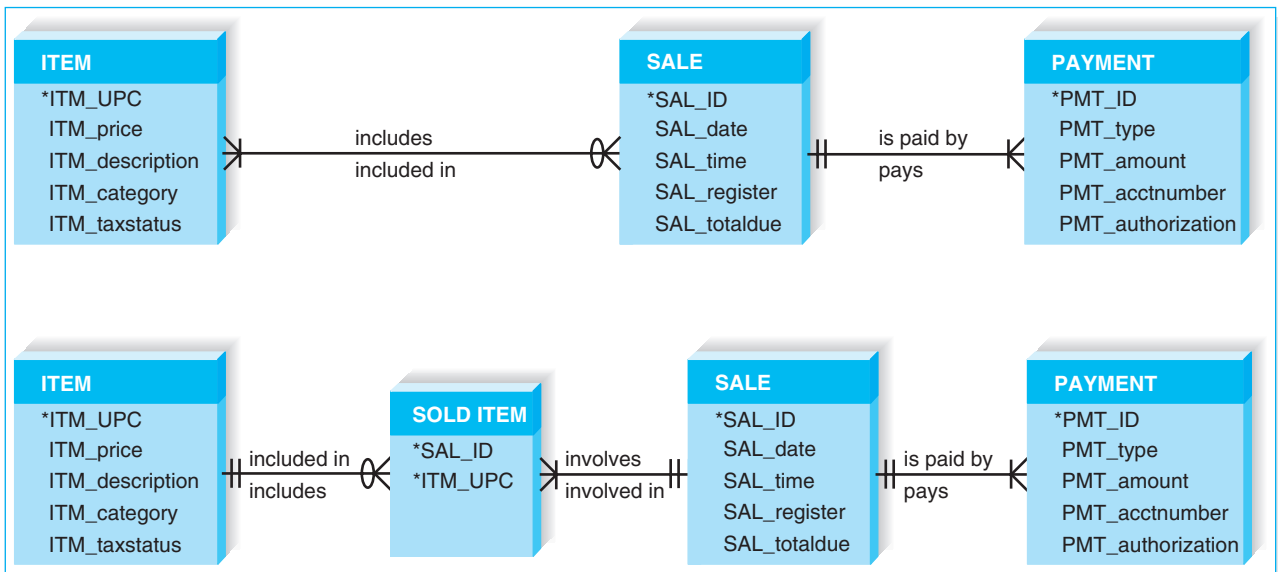
FIGURE 6-12 Resolving an M:N Relationship
