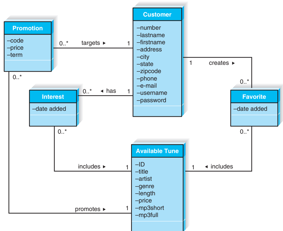
FIGURE 14-21 Revised Attributes and Associations
