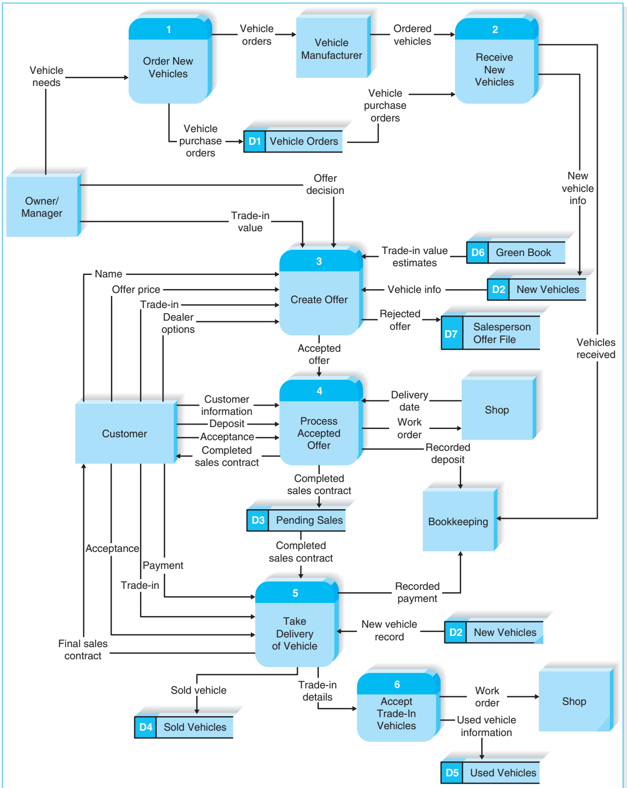
FIGURE 5A-3 Holiday Travel Vehicles Level 0 DFD
