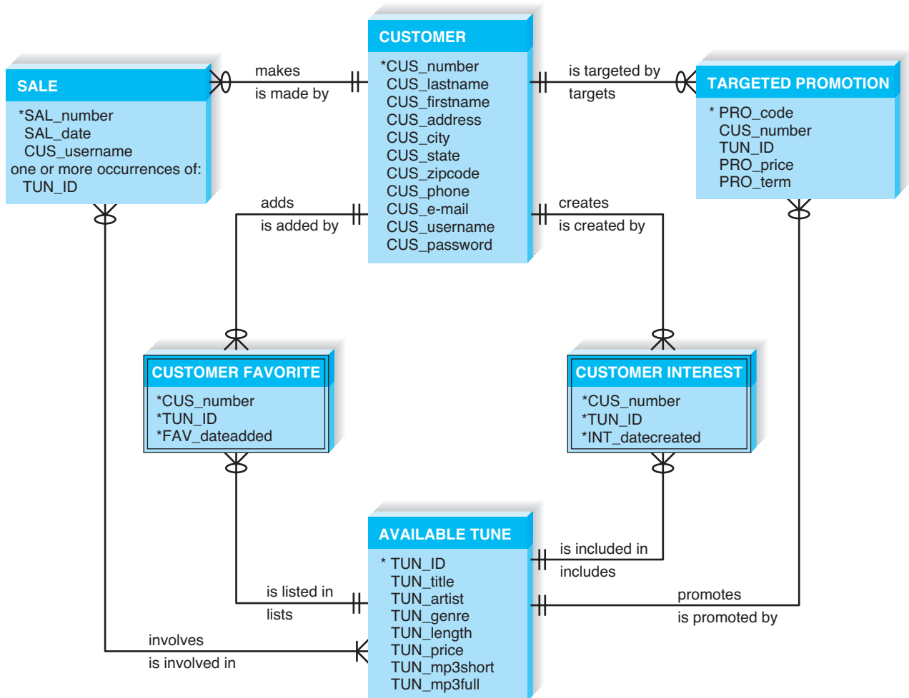
FIGURE 6-15 Relationships for Tune Source ERD
