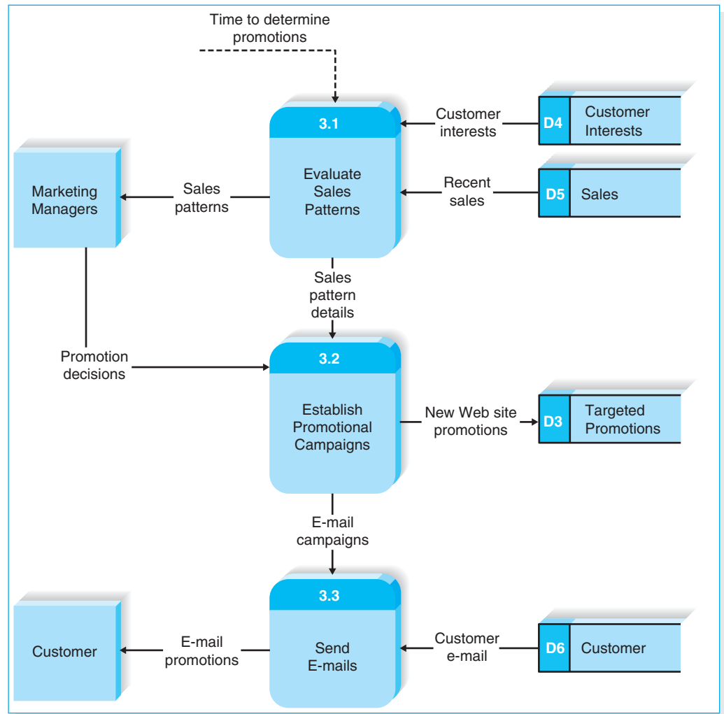
FIGURE 5-18 Level 1 DFD for Tune Source Process 3: Promote Tunes
