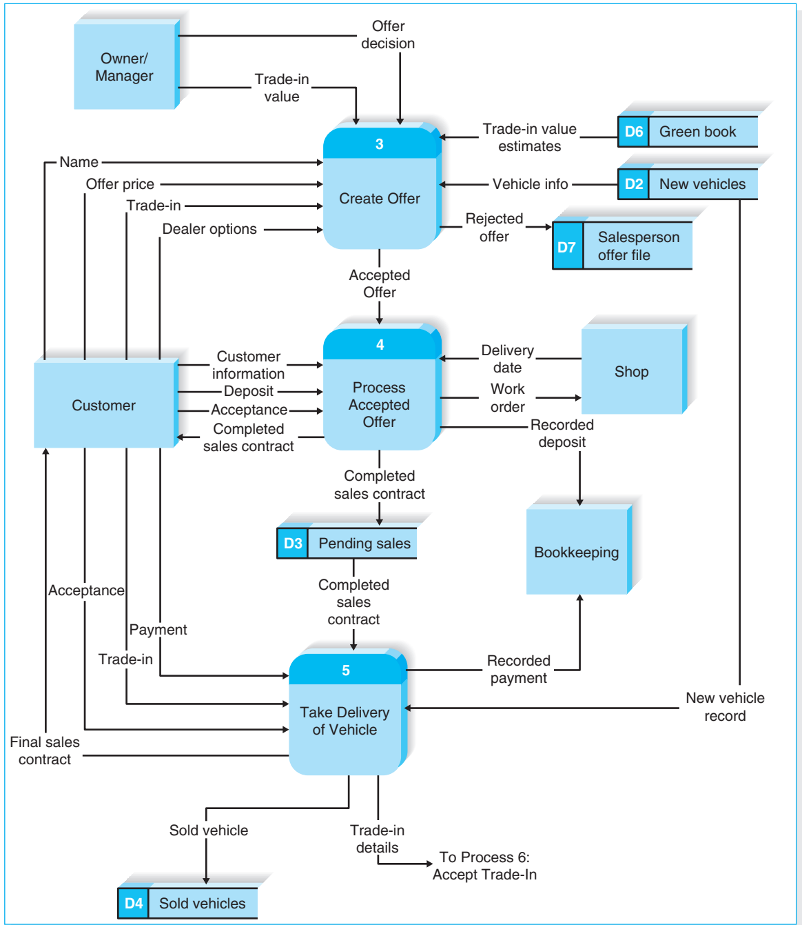
FIGURE 5-8 Holiday Travel Vehicles Partial Level 0 DFD
