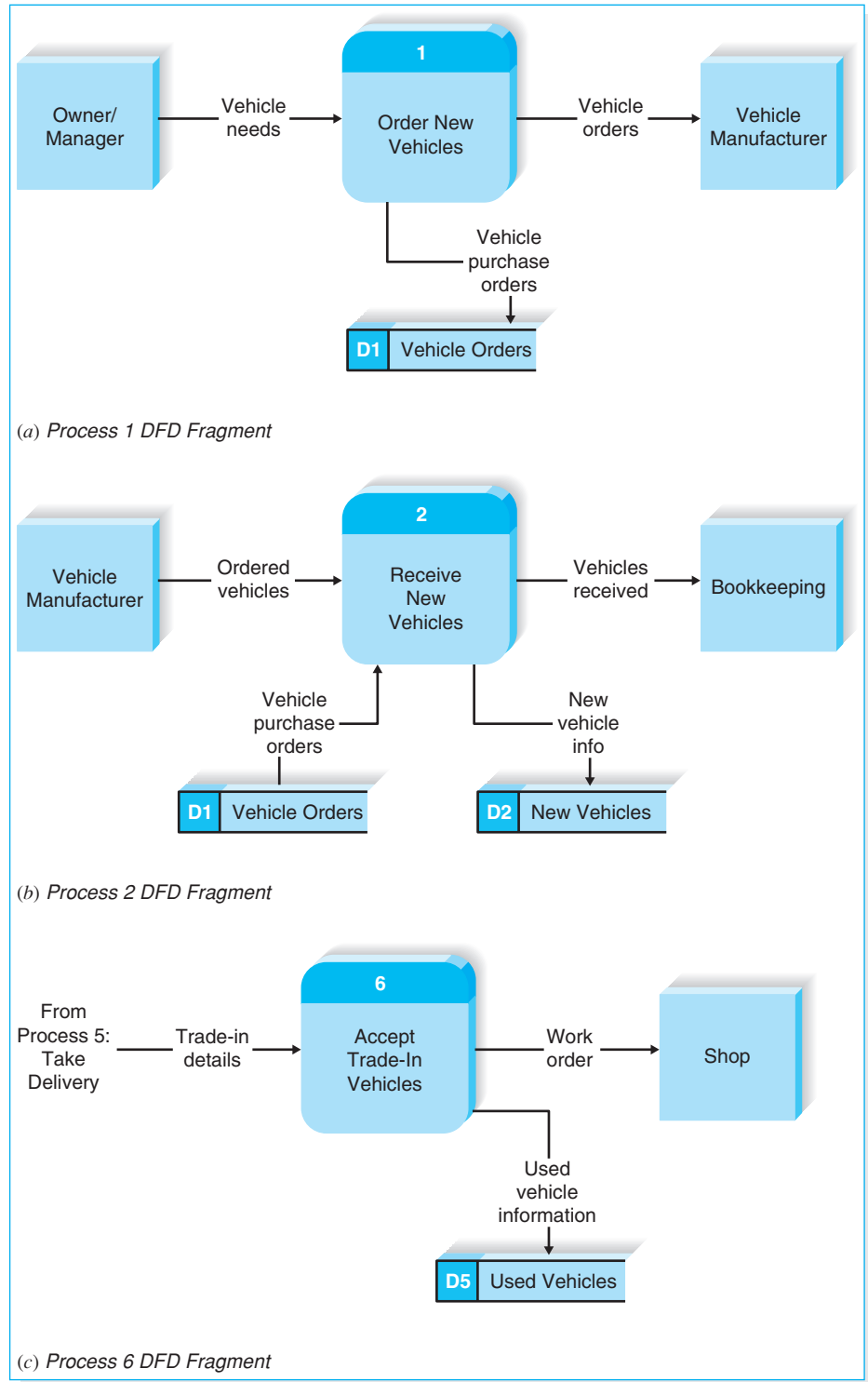
FIGURE 5A-2 Additional DFD Fragments for Holiday Travel Vehicles
