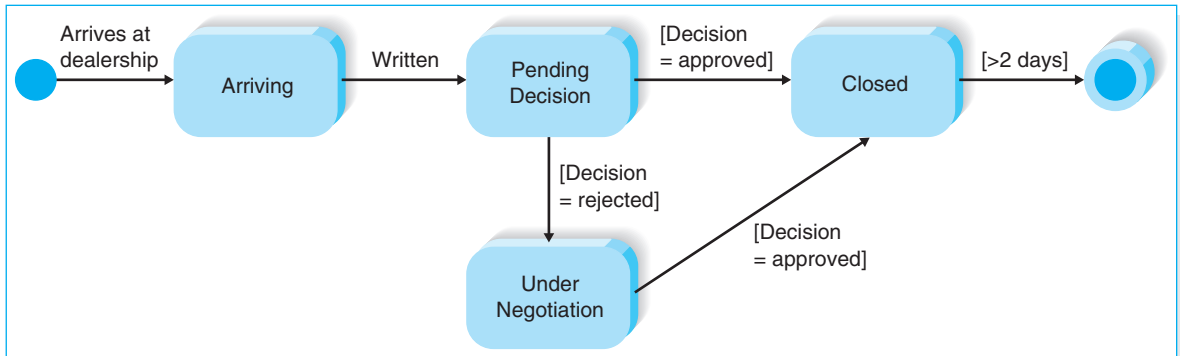
FIGURE 14-26 Behavioral State Machine Diagram for an Offer for a Vehicle
