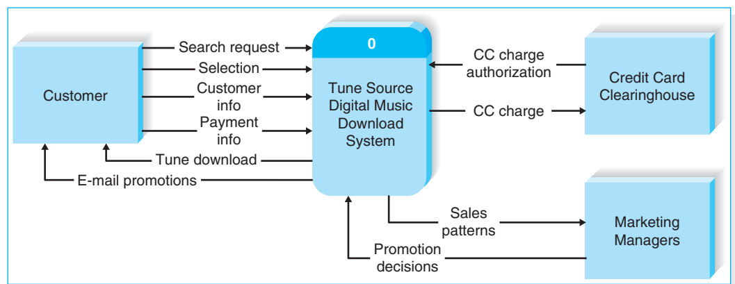
FIGURE 5-13 Tune Source Context Diagram
