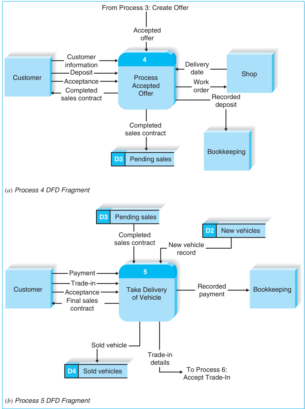
FIGURE 5-7 Additional DFD Fragments for Holiday Travel Vehicles
