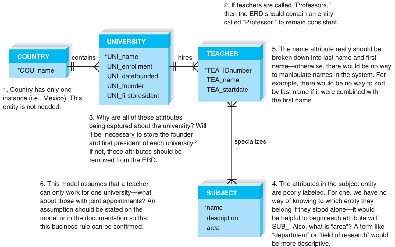
FIGURE 6-16 Data Modeling Guidelines Summary
