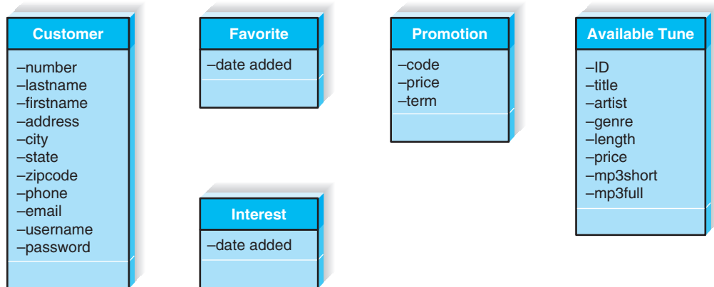
FIGURE 14-20 Initial Attributes for Class Diagram
